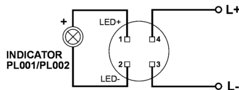
Figure-2- Indicator Connection
