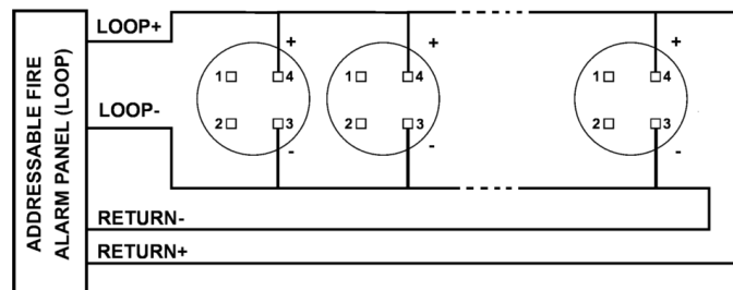
Figure-1- Loop Connection
